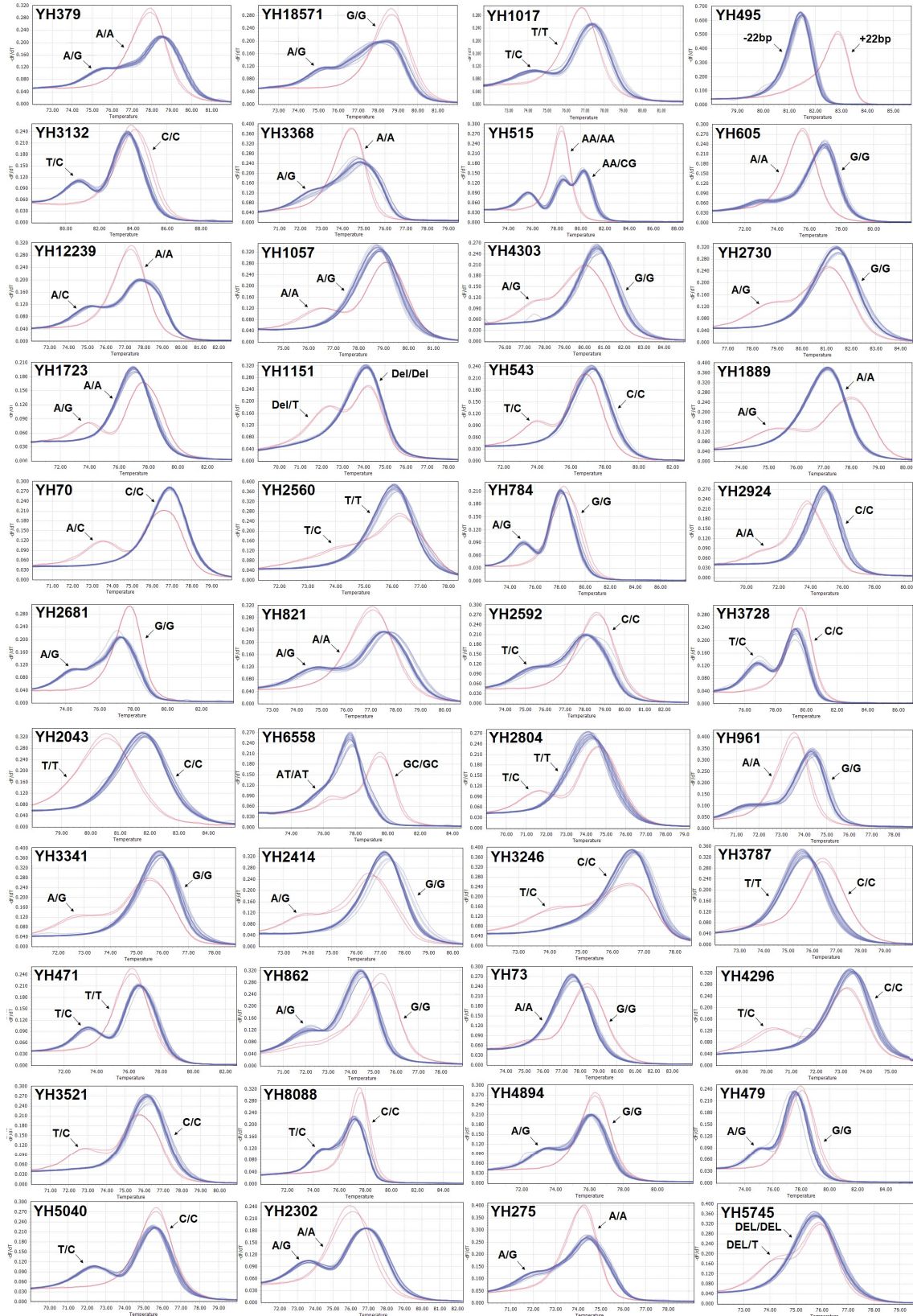
Supplementary Fig. 5. Normalized melting peak patterns of 44 high resolution melting (HRM) makers developed in this study. Detail information about HRM markers is shown in Supplementary Table 6.
