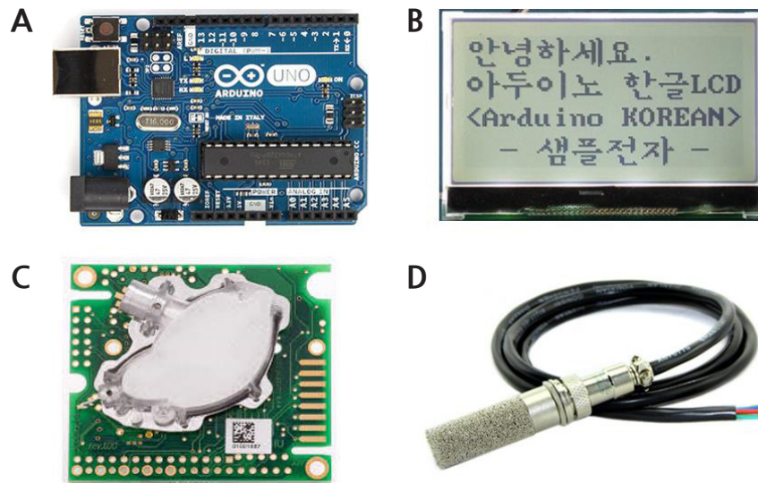
Fig. 1. Open-source prototype board(Arduino Uno, Arduino, Ivrea, Italy, A), 128x64 graphic LCD(SE-KLCD-A, Sample Electronics, Korea, B), CO 2 meter(SE-0018, CO 2 Meter, Inc, FL, USA, C), and soil temperature/moisture sensor(SHT10, Adafruit Industries, NY, USA, D).
